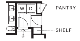
* A1 PLAN MUD/LAUNDRY IN UNITS 21, 25 & 29
